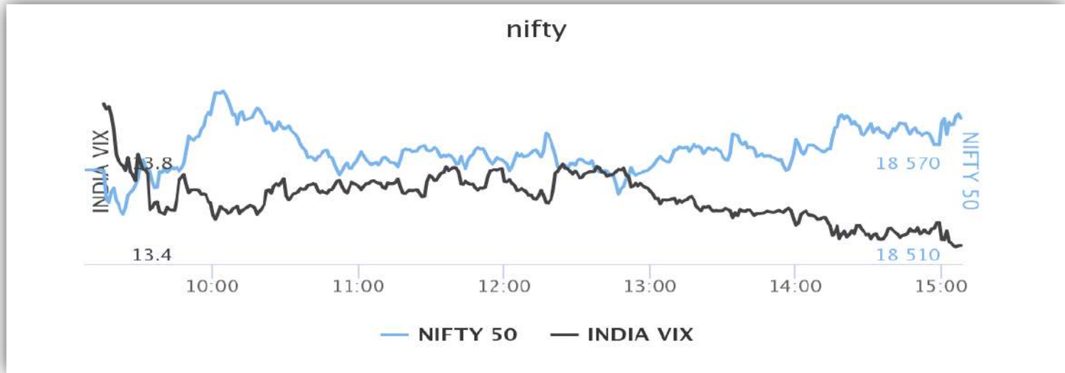
Nifty50 Chart (08-12-2022)
